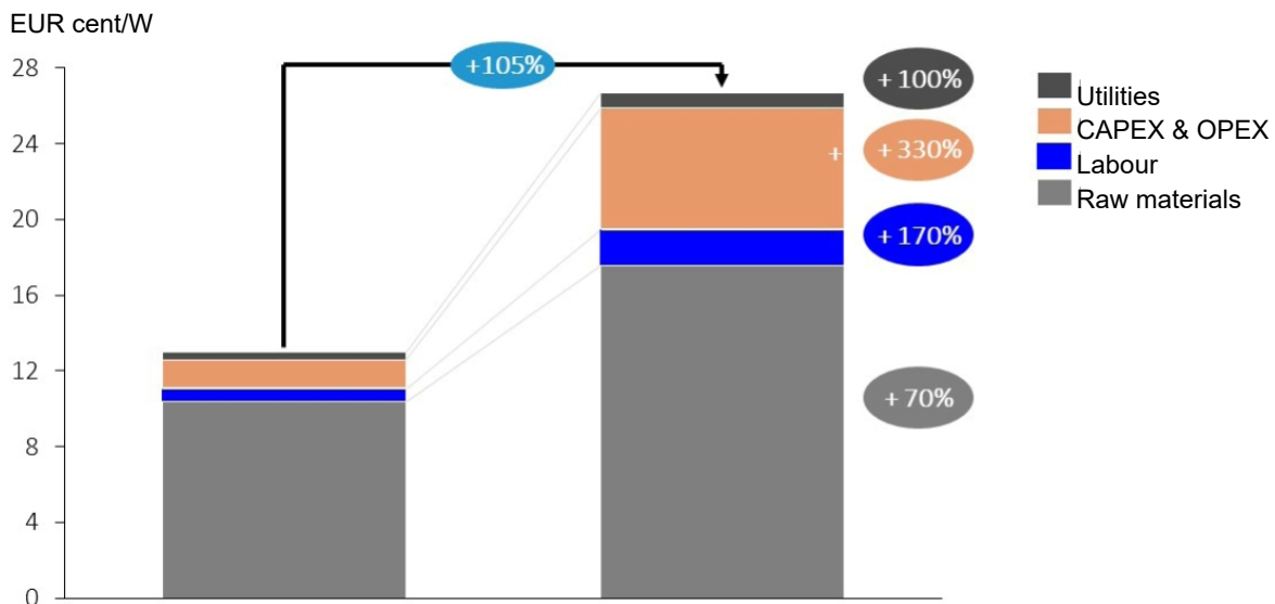
FIGURE 7 Observed cost structure comparison in integrated cell and module manufacturing (EUR cent/W)
