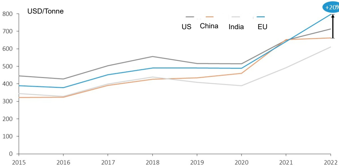
FIGURE 4 Example steel: hot rolled coil production costs
